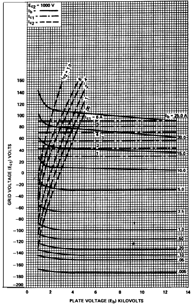
Figure 5 - Typical Constant Current Tube Characteristics @ E_{c2} = 1000 V
