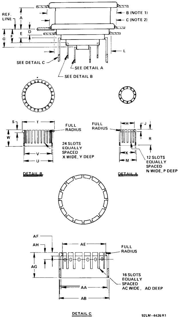
Figure 9 - Preferred Mounting Arrangement
