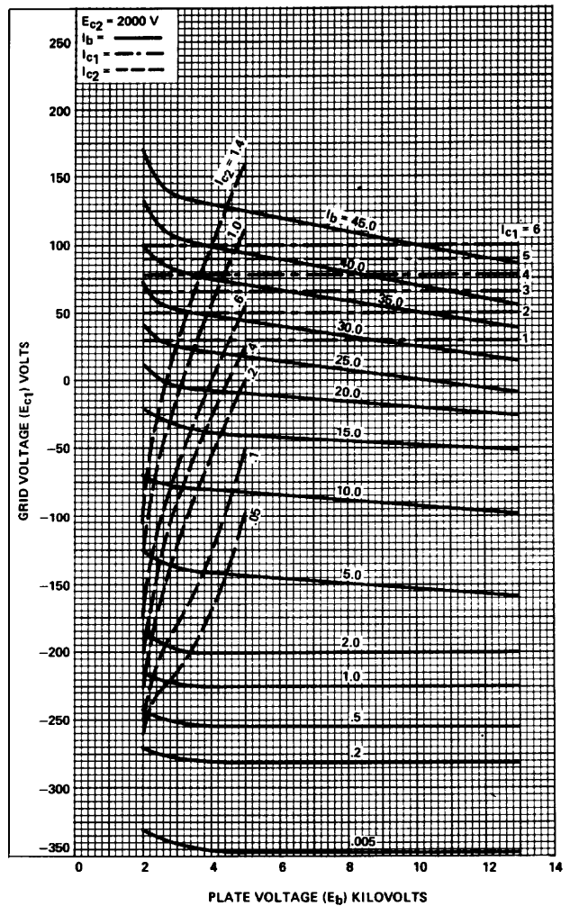
Figure 3 - Typical Constant Current Tube Characteristics @ E_{c2} = 2000 v
