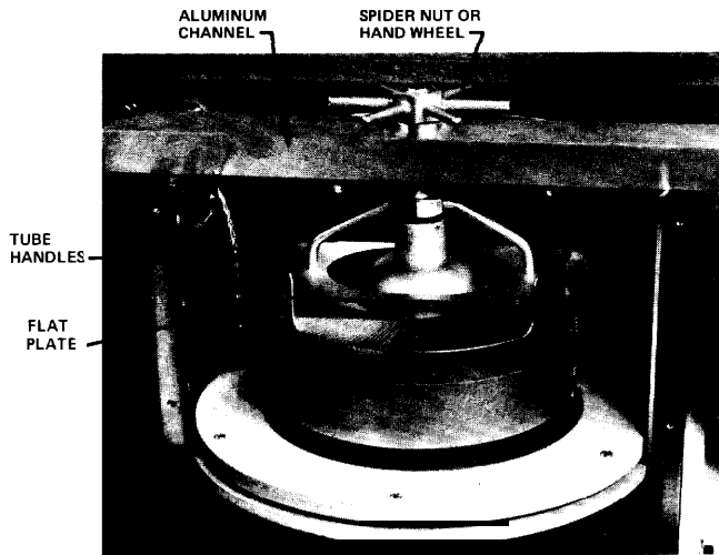
Figure 10 - Tube Removal Assembly
