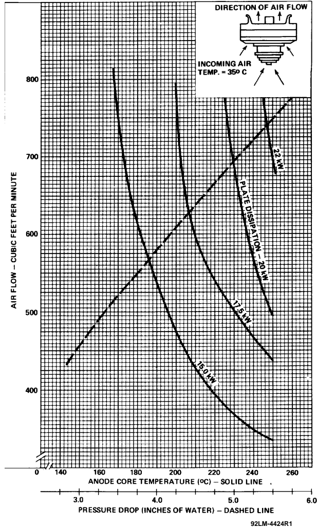
Figure 7 - Typical Cooling Characteristics
