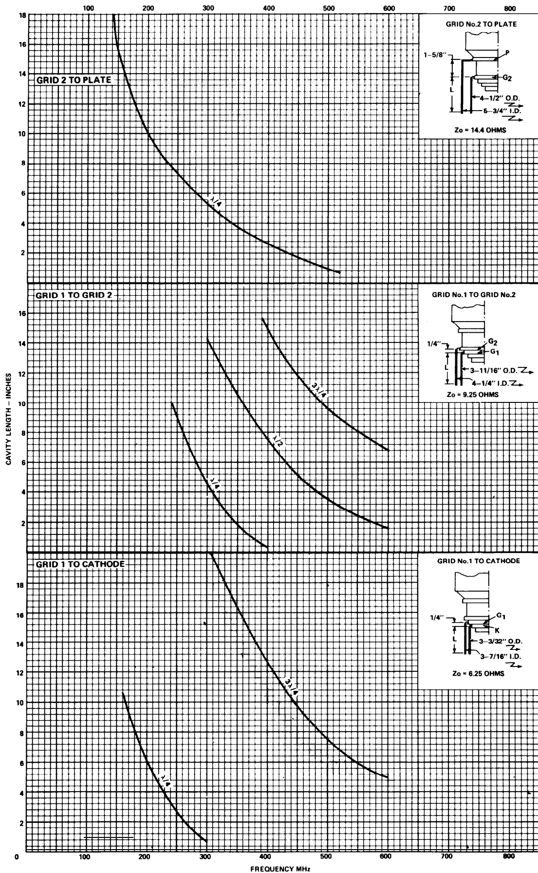
Figure 6 - Electrode Cavity Tuning Characteristics
